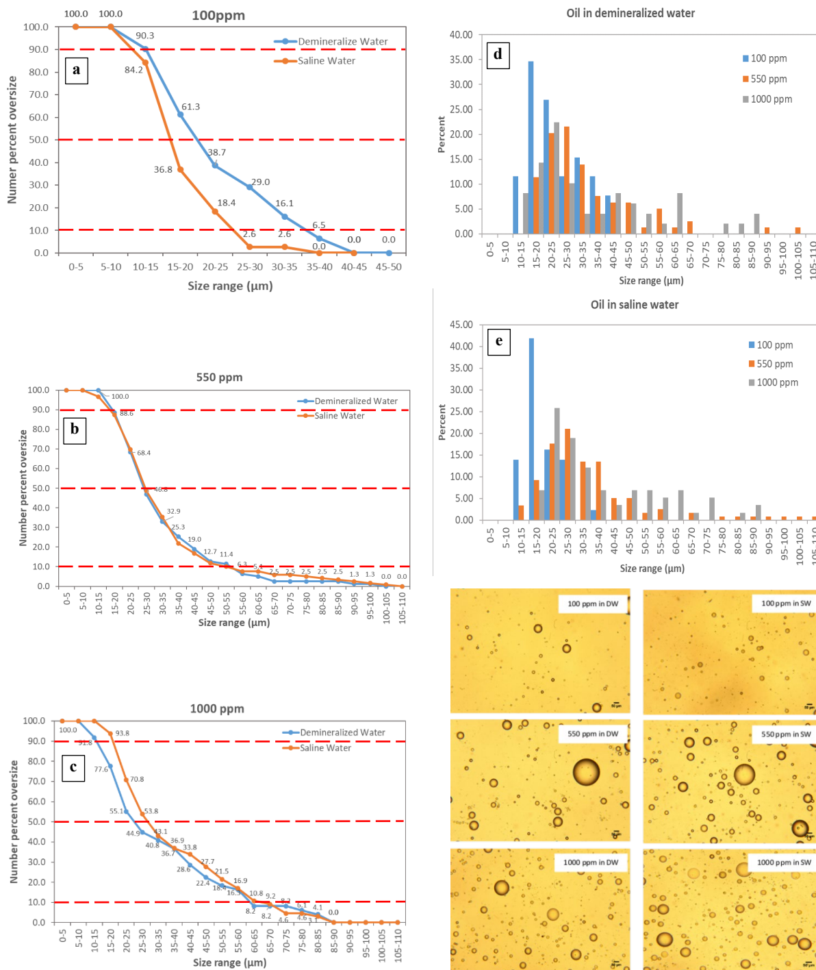
Fig. 2. Microscopic images, cumulative size distribution of oil droplets dispersed in DW and SW before IGF. Note. (a) 100 ppm, (b) 550 ppm, and (c) 1000 ppm oil, and differential size distributions of 100, 550, 1000 ppm oil, (d) DW, and (e) SW.
