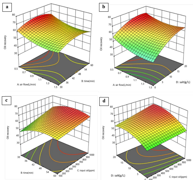
Fig. 6. 3D Surface plots illustrating the effect of air flow rate, processing time, salt concentration, and input oil concentration on the percent of oil separation efficiency.
