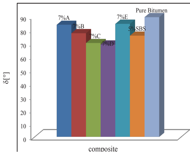
Fig. 8. Phase angle shift of the pure bitumen and the modified ones at 80.1 °C.
